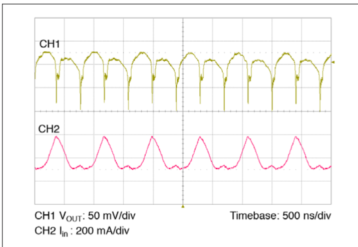
Figure 9 — Full load ripple, 100 \mu\text{F } C_{IN} ; No external C_{OUT} . Board mounted module, scope setting: 20 MHz analog BW
