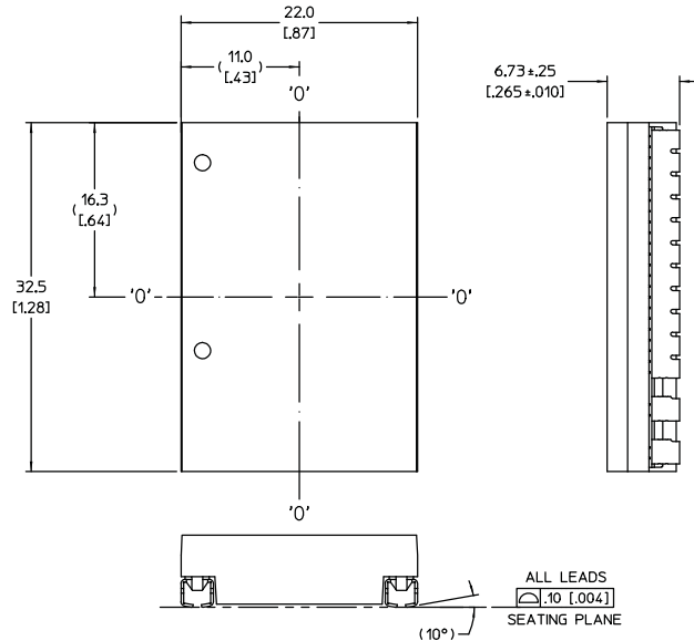
TOP VIEW (COMPONENT SIDE)
