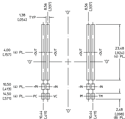
RECOMMENDED LAND PATTERN (COMPONENT SIDE SHOWN)
